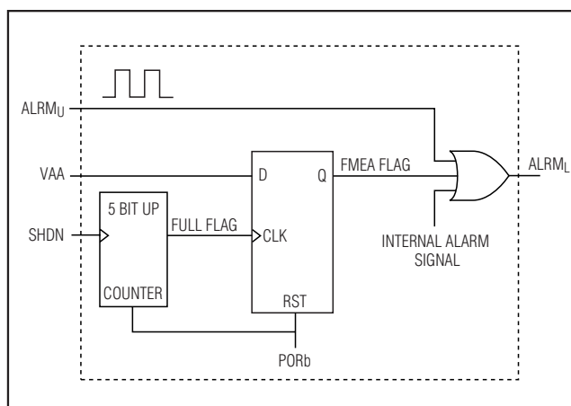
Figure 18. Internal FMEA \overline{\text{SHDN}} Pin Functionality Circuit
