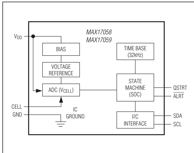
Figure 2. Block Diagram
