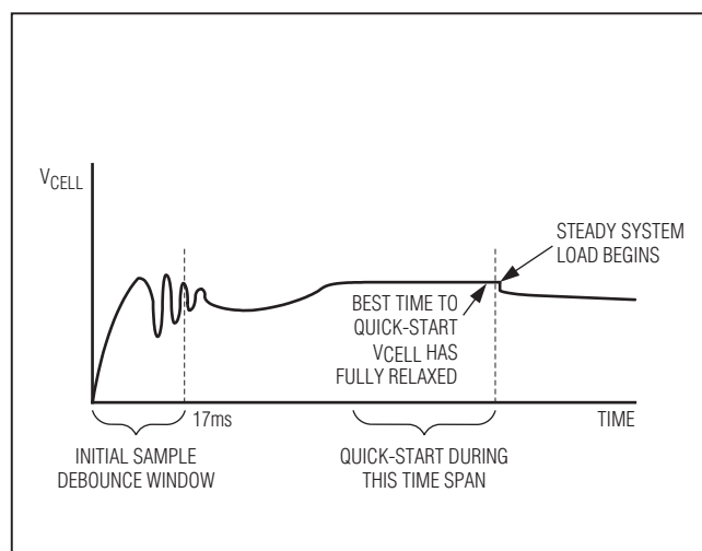
Figure 7. Insertion Waveform Requiring Quick-Start Command
