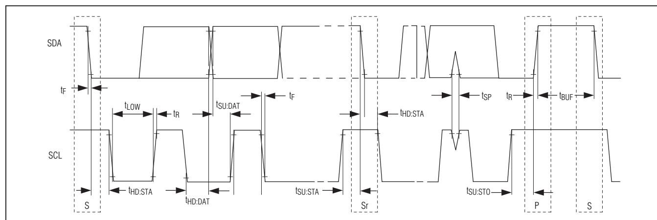
Figure 1. I 2 C Bus Timing Diagram
