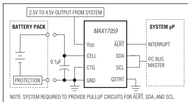
Figure 13. MAX17059 Application Circuit (2S Cell Pack)
