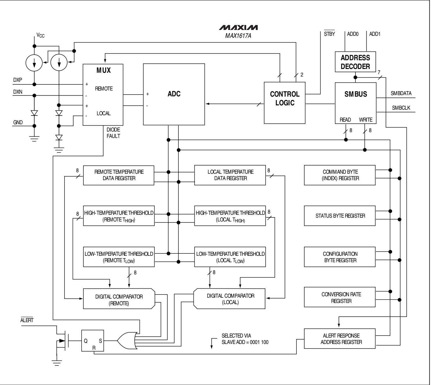
Figure 1. Functional Diagram
