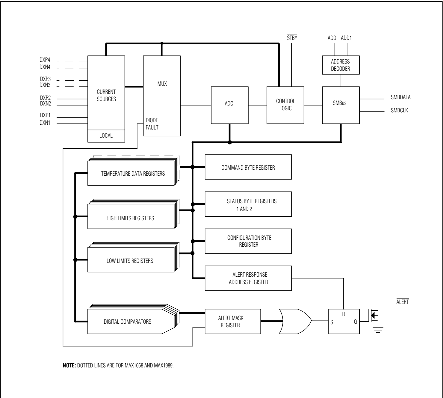
Figure 1. MAX1668/MAX1805/MAX1989 Functional Diagram
