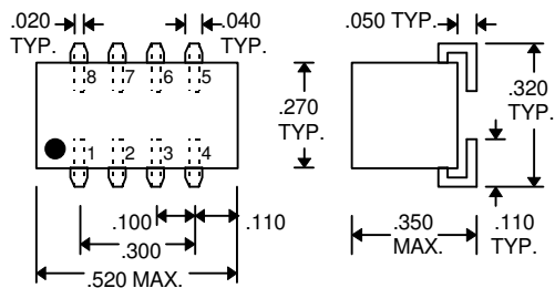
MDU28C-xxB1 (Commercial J-Lead)
