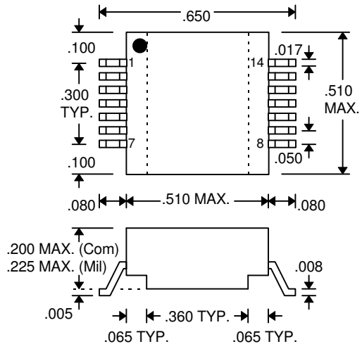
MDU28C-xxD4 (Commercial SMD) MDU28C-xxMD4 (Military SMD)
