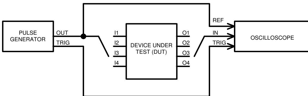
Test Setup
