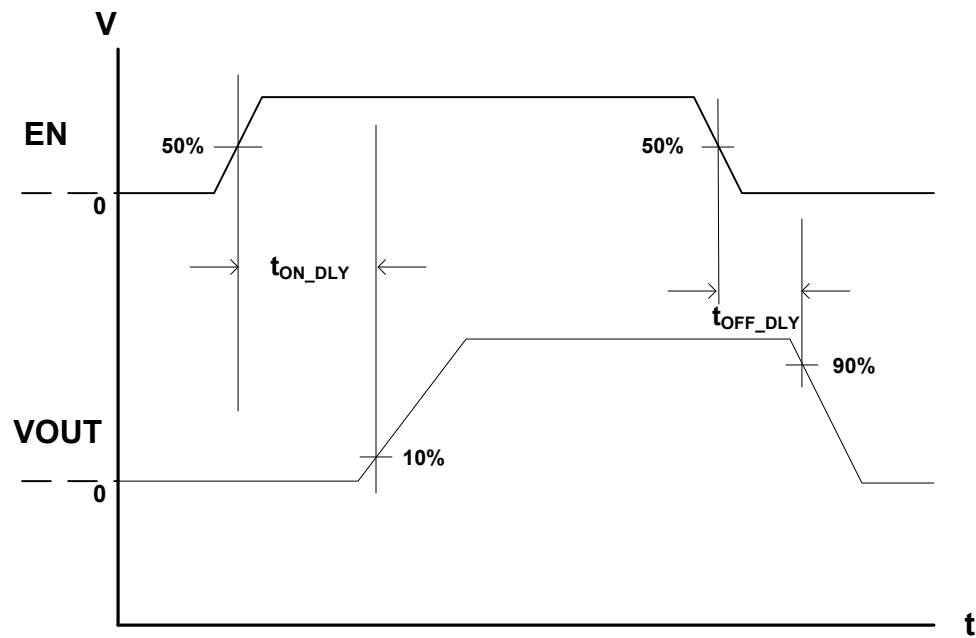
Figure 2. Turn-On/Off Delay
