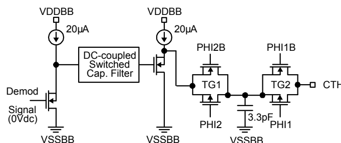
Figure 2. CTH Pin
