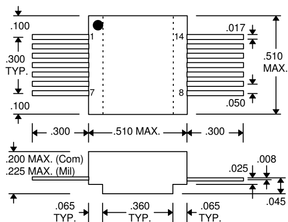
DLO31F-xxD1 (Commercial SMD) DLO31F-xxMD1 (Military SMD)
