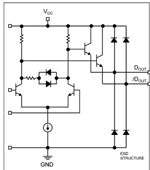
Figure 3. Output Structure
