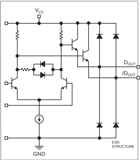
Figure 3. Output Structure
