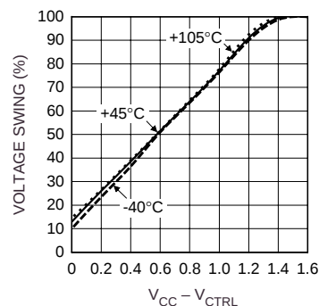
Typical Voltage Output Swing V_{CC} = 3.3V or 5V
