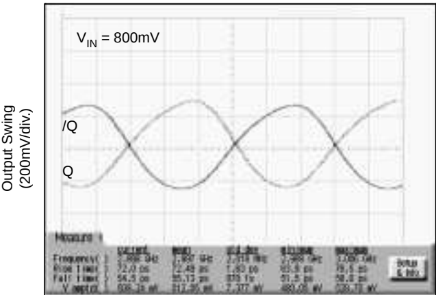
3.0GHz Output
