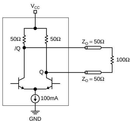
Figure 2b. CML DC-Coupled (100Ω Termination)
