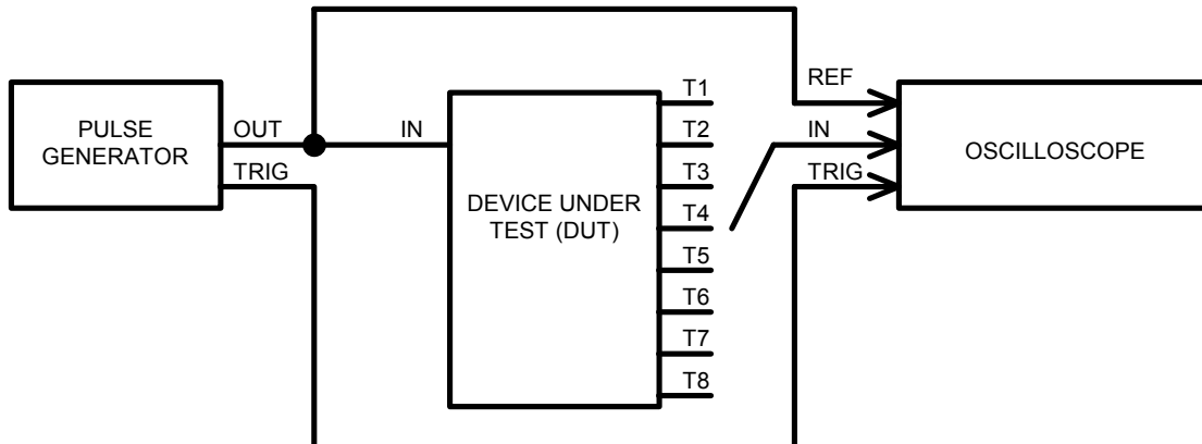
Test Setup
