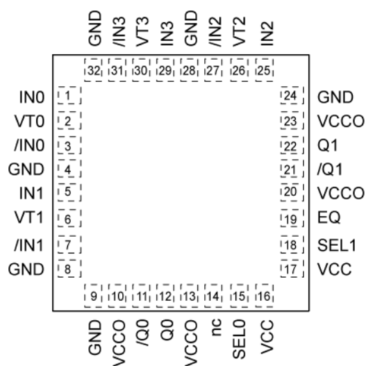
32-Pin QFN
