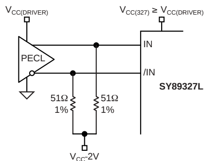
Figure 7. PECL-DC Coupled
