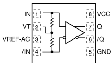
8-Pin DFN
