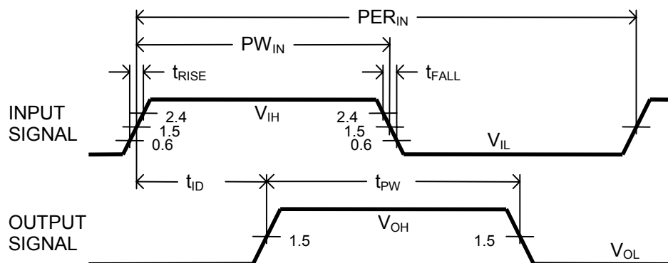
Figure 8: Timing Diagram
