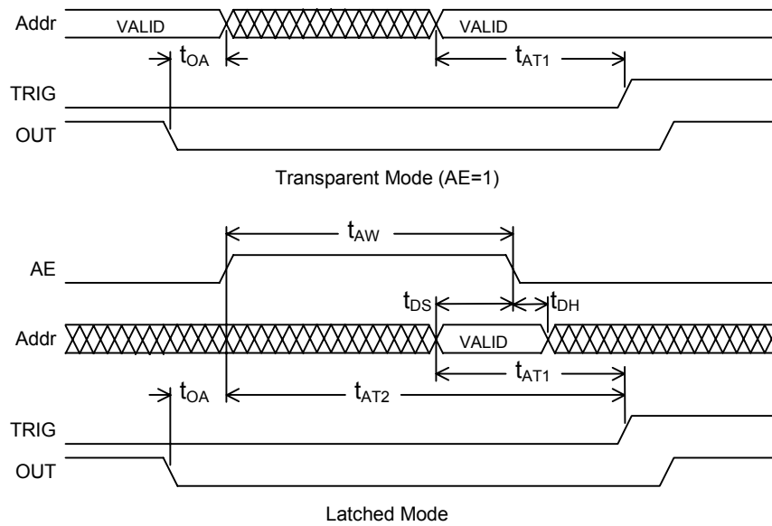
Figure 4: Address Update
