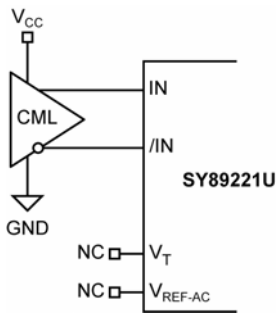
Figure 4a. CML Interface (DC-Coupled) May connect V_T to V_{CC}
