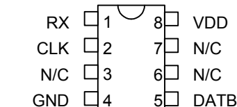
3D7522Z-xxx SOIC (.150)
