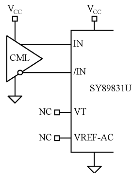
Figure 3c. DC-Coupled CML Input Interface
