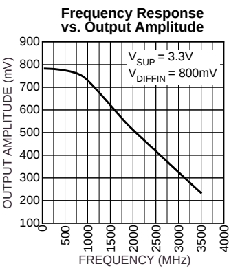
Frequency Response vs. Output Amplitude @3.3V
