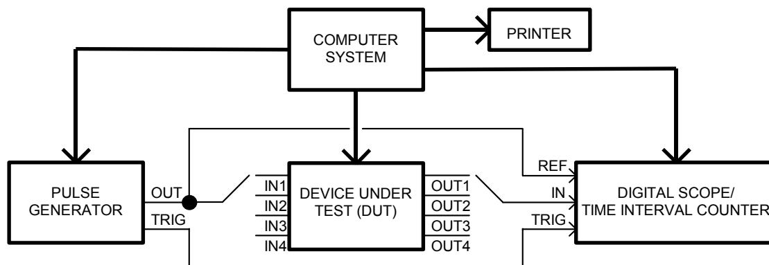
Figure 4: Test Setup
