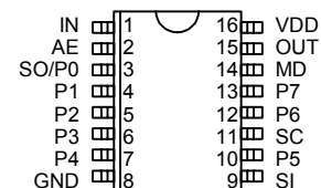
3D7408S SOL (300 Mil)
