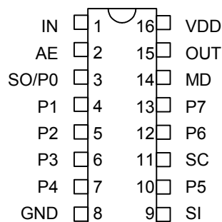
3D7408 DIP 3D7408G Gull Wing
