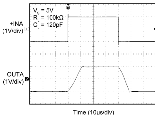
Large Signal Step Response (Non-Inverting)
