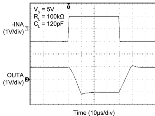
Large Signal Step Response (Inverting)
