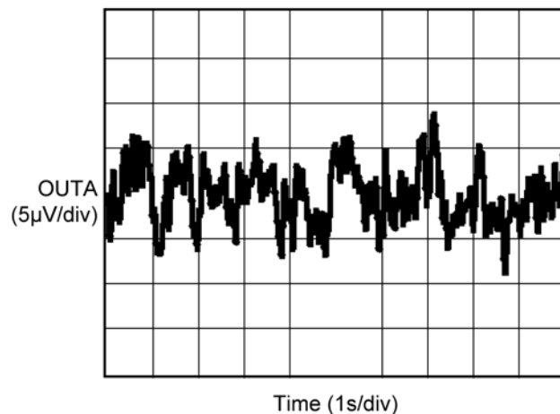
0.1Hz to 10Hz Input Referred Voltage Noise
