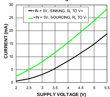
Short Circuit Current vs. Supply Voltage
