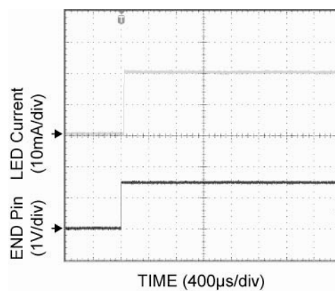
Figure 10. PWM Signal at 100% Duty Cycle ( I_{avg} = 20mA )
