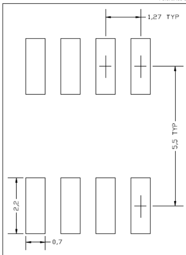
8-Pin SOIC
