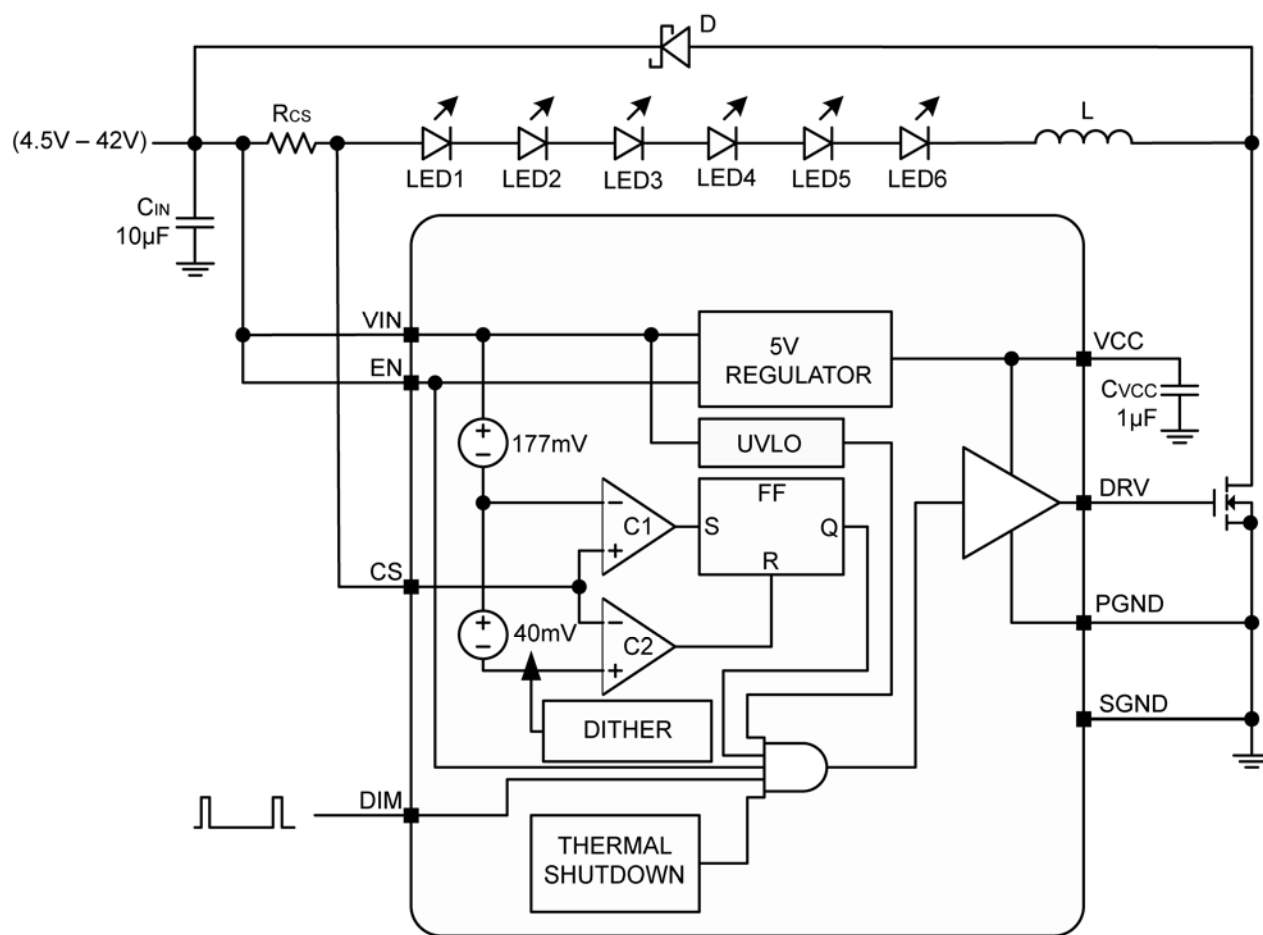
Figure 1. MAQ3203 Block Diagram
