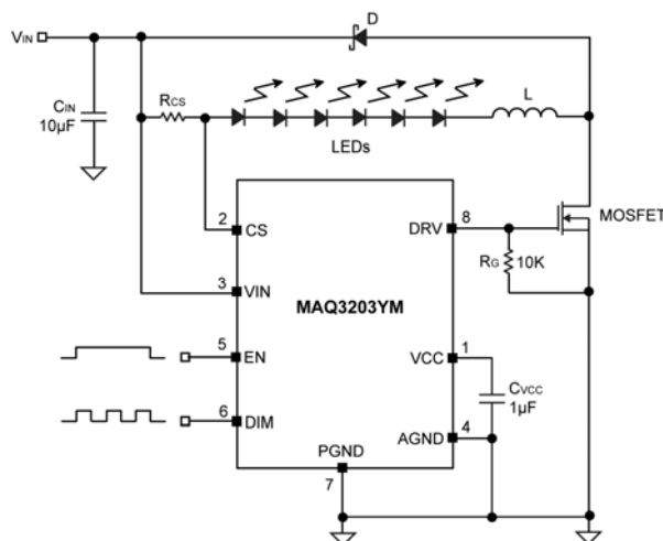
MAQ3203 Step-down LED Driver
