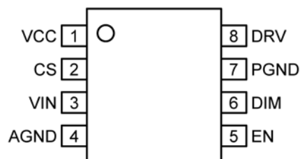
8-Pin SOIC MAQ3203
