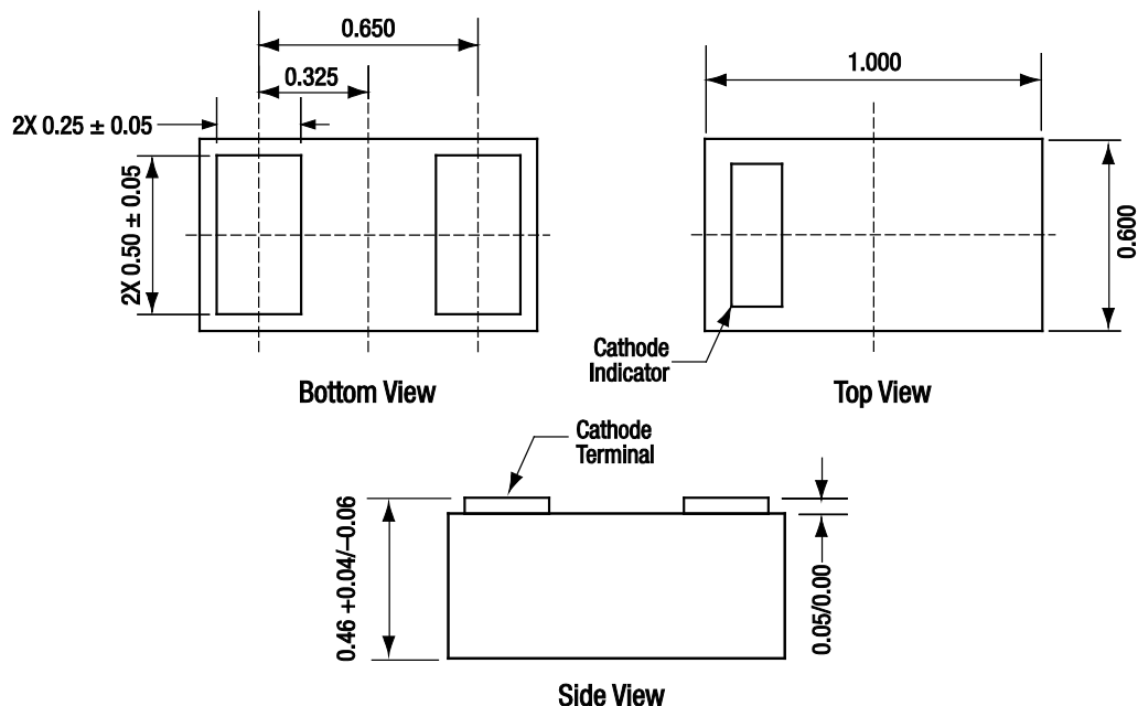
Figure 6. SMV1235-040LF Package Dimensions
