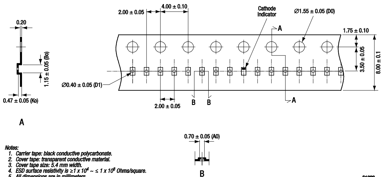
Figure 7. SMV1235-040LF Tape and Reel Dimensions
