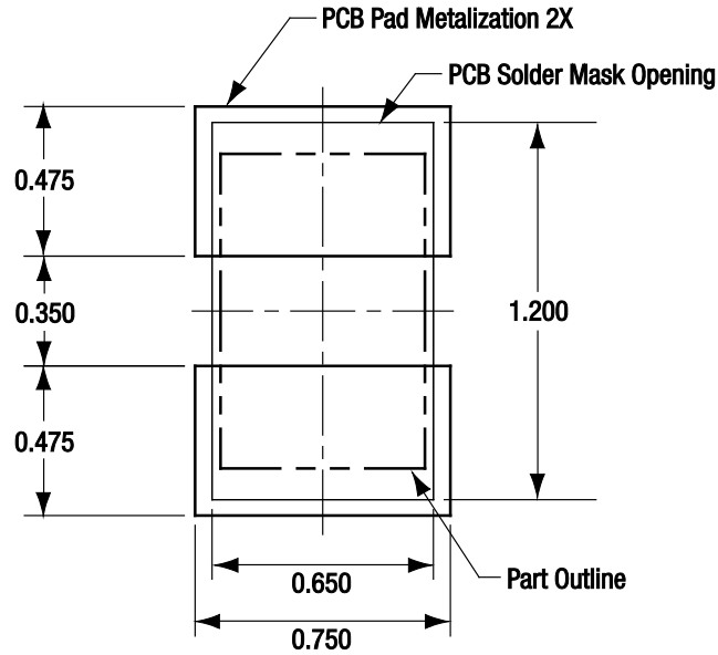
Figure 4. SMV1235-040LF PCB Layout Footprint
