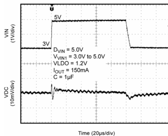
LDO Line Transient
