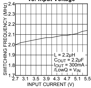
Line Regulation
