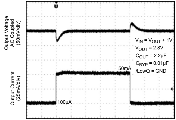
LDO2 Load Transient LowQ Mode
