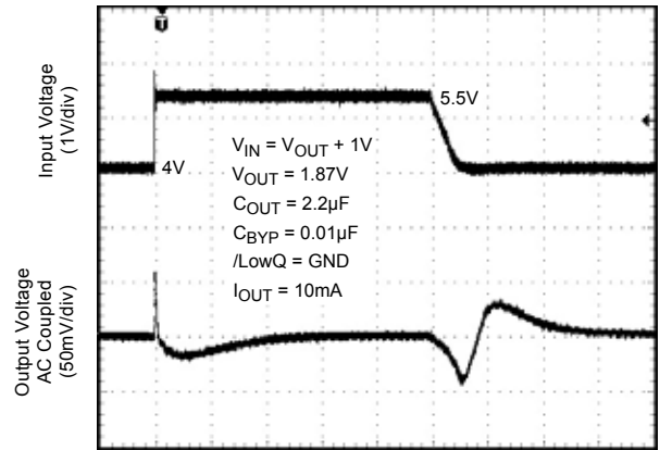
LDO2 Line Transient LowQ Mode
