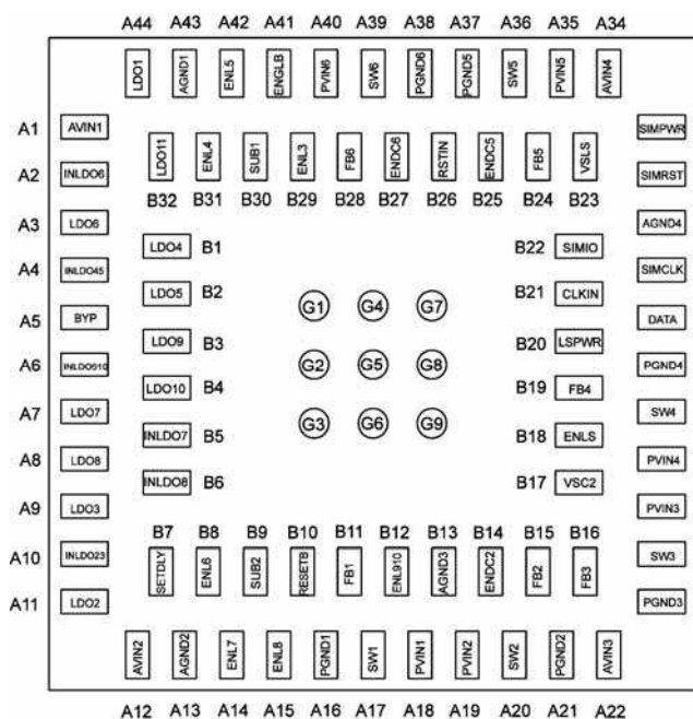
76-Pin 5.5mm x 5.5mm LGA Package (AL)
