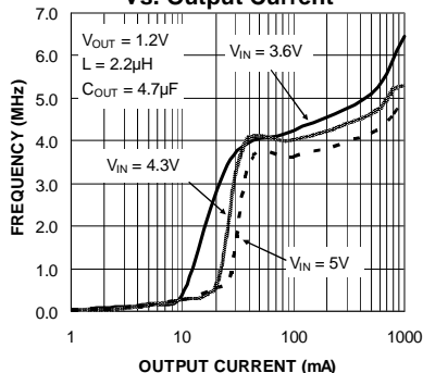
DC4 HLL SW Frequency vs. Output Current
