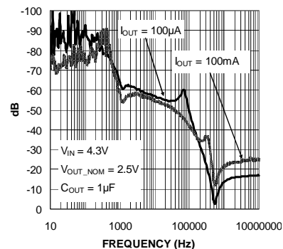
Typical LDO PSRR
