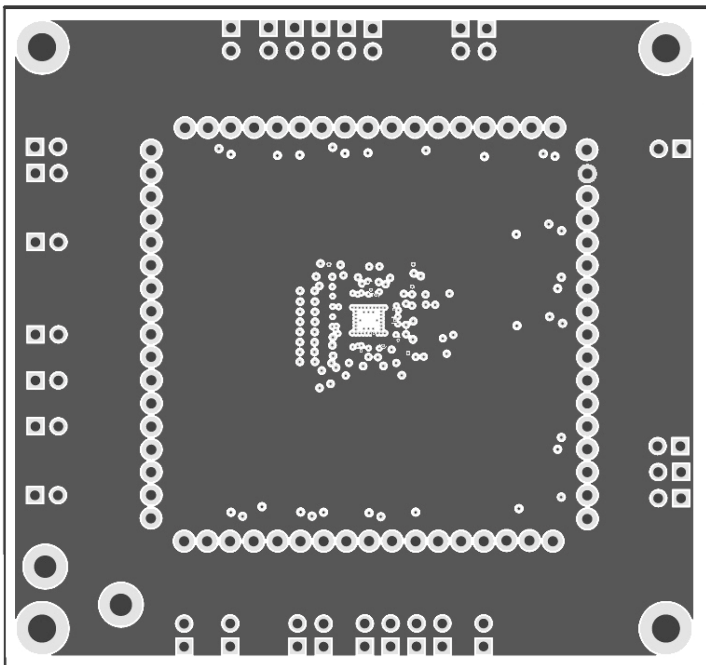
FBGA/LGA DC Regulator AGND (Layer 5)
