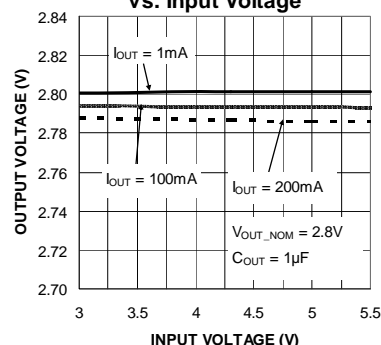
LNR6 Output Voltage vs. Input Voltage
