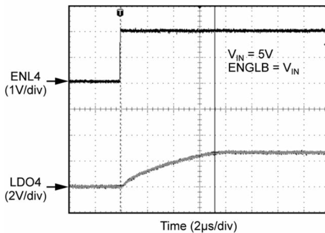
Start-Up Waveform for Typical LDO
