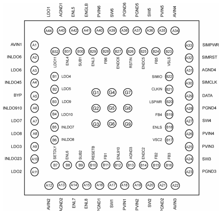
85-Pin 5.5mm x 5.5mm FBGA Package (AB)
