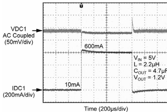
Load Transient HLL DC1 10mA to 600mA
