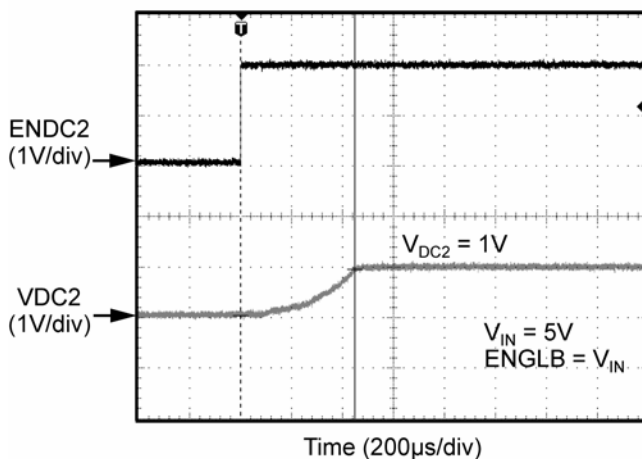
Start-Up Waveform for DC2
