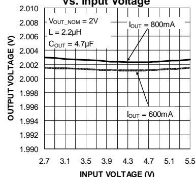
LDO3 Output Voltage vs. Input Voltage
