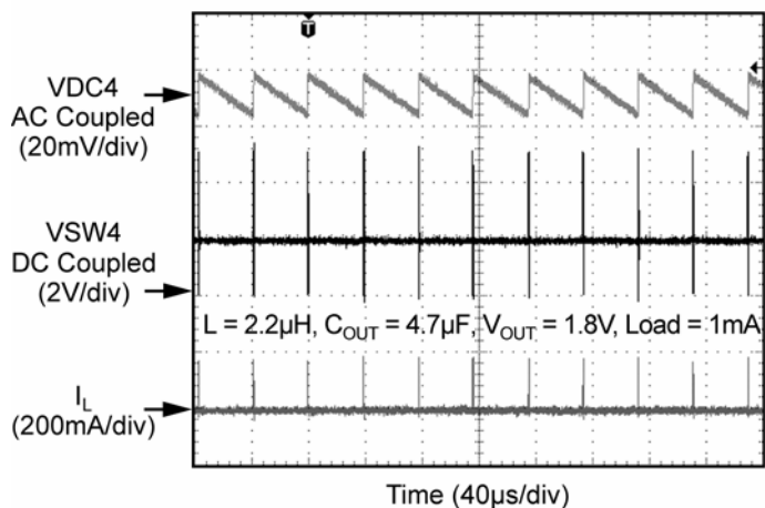
4MHz HLL Switching Waveform at 1mA
