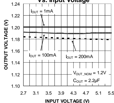
LNR9/10 Output Voltage vs. Input Voltage
