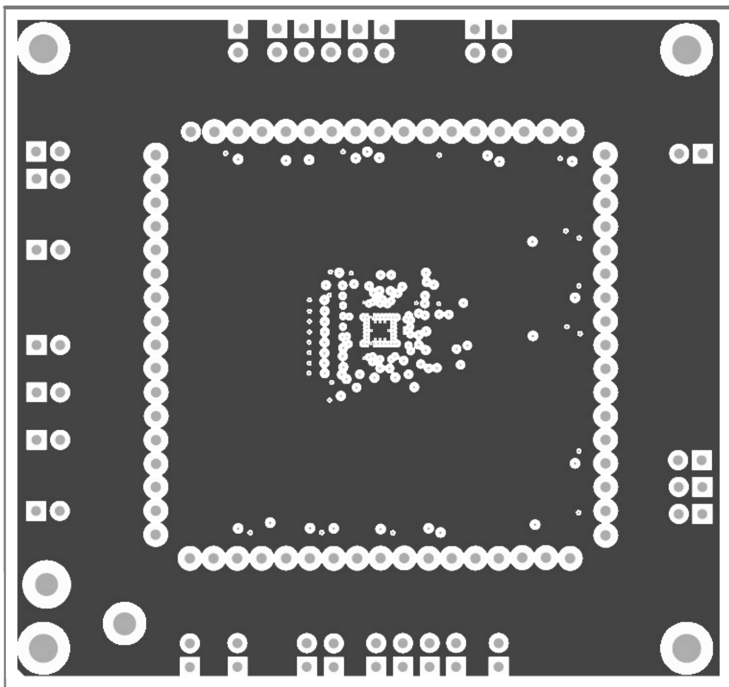
FBGA/LGA LDO GND (Layer 7)
