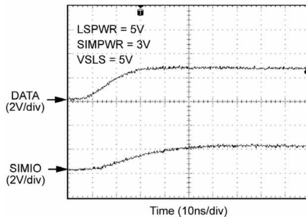
DATA to SIMIO Rise Time
