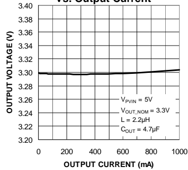
DC5 Output Voltage vs. Output Current
