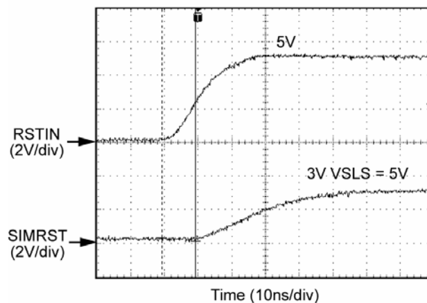
RSTIN to SIMRST Rise Time
