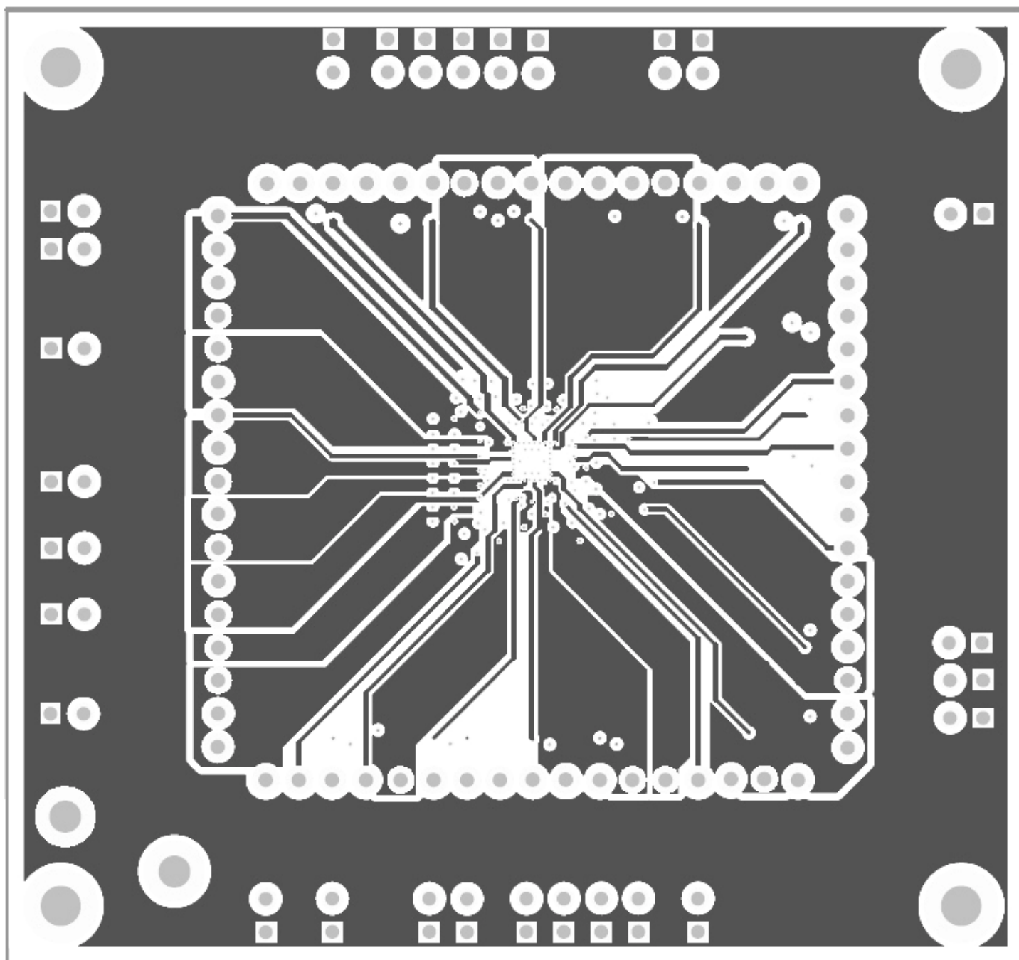
FBGA/LGA Power and Signal (Layer 3)
