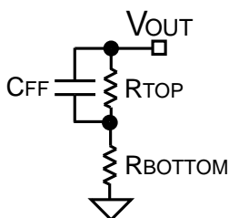
Figure 2. Feedback Resistor Network
