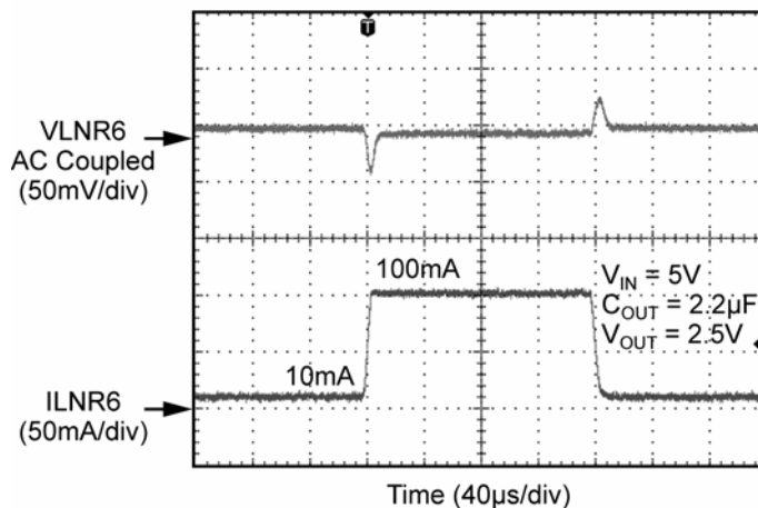
LNR6 Load Transient 10mA to 100mA
