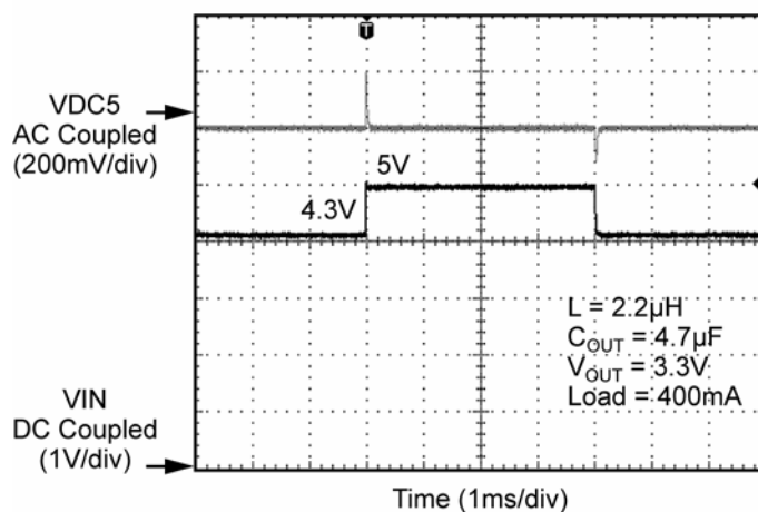
DC5 Line Transient
