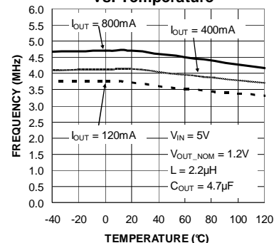
4MHz HLL SW Frequency vs. Temperature
