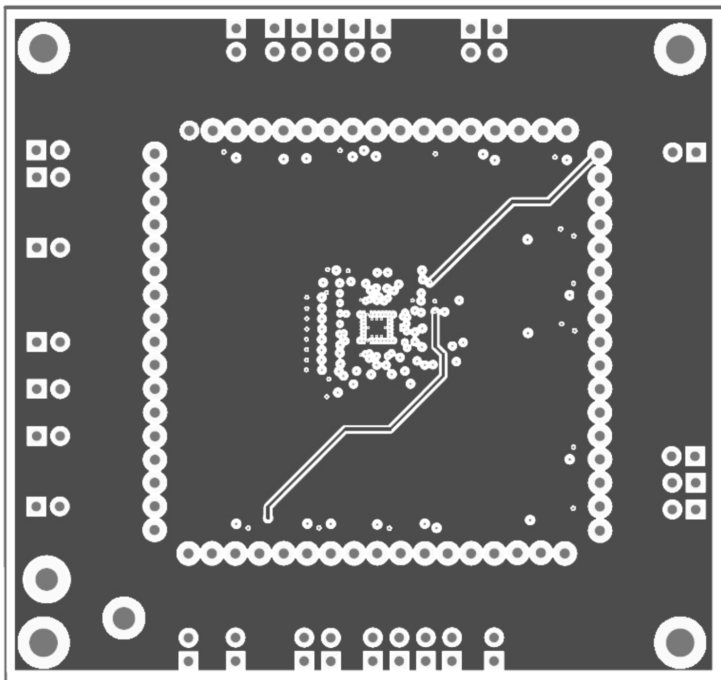
FBGA/LGA LDO GND (Layer 2)
