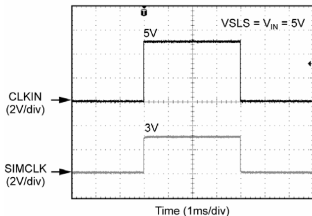
CLKIN to SIMCLK Level Translation
