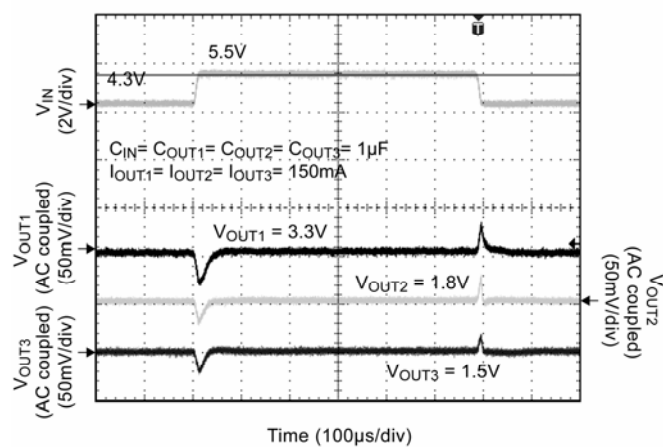
Line Transient
