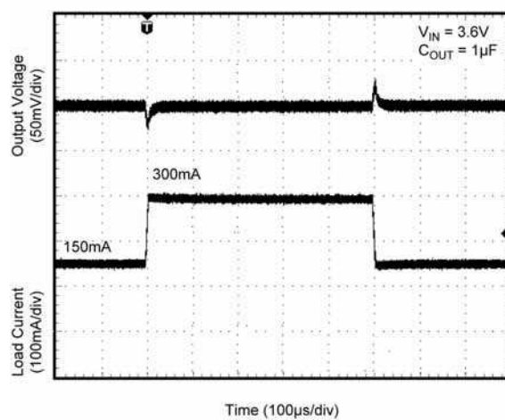
Load Transient
