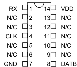
3D3522D-xxx SOIC (.150)
