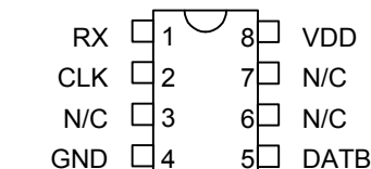
3D3522Z-xxx SOIC (.150)
