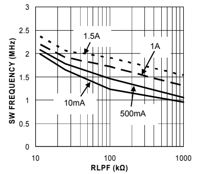
Switch Frequency vs. RLPF Resistance (5.0V-1.0V)
