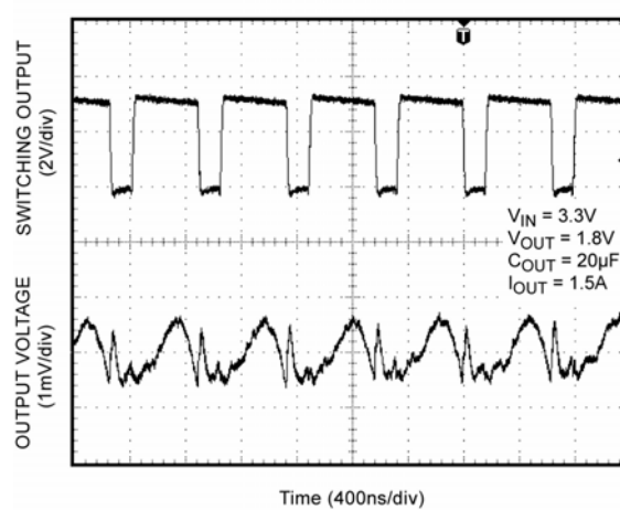
Output Ripple
