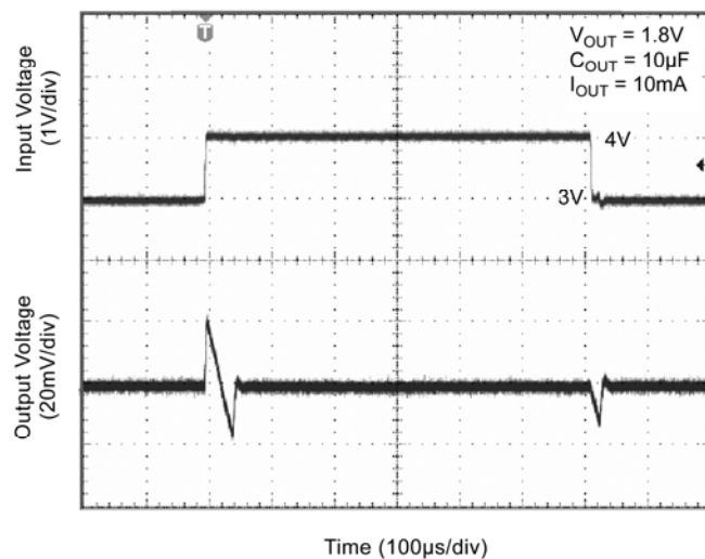
Line Transient
