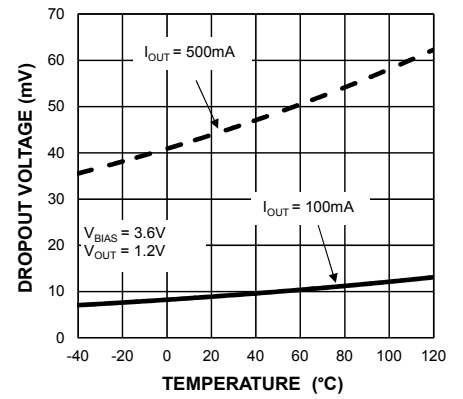
Input Dropout Voltage vs. Temperature
