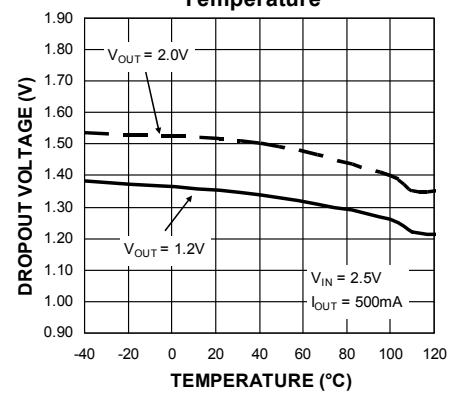
Bias Dropout Voltage vs. Temperature
