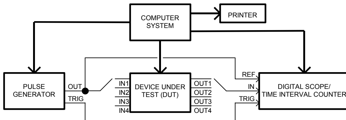
Figure 4: Test Setup
