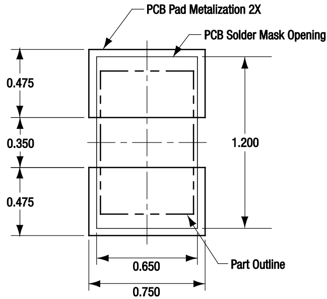
Figure 4. SMV1405-040LF PCB Layout Footprint
