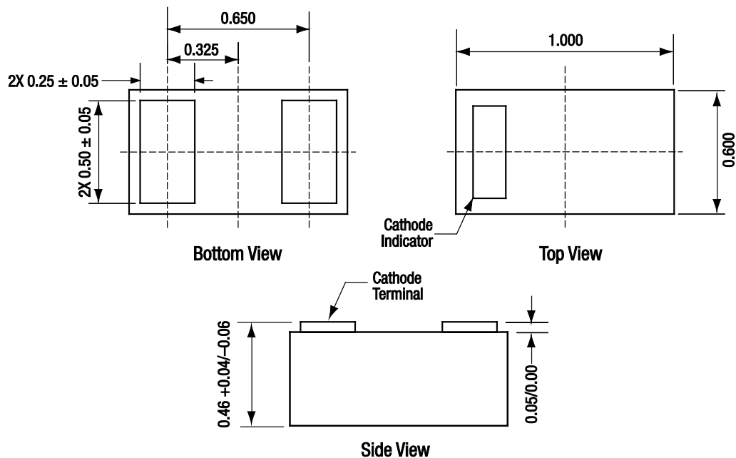
Figure 6. SMV1405-040LF Package Dimensions
