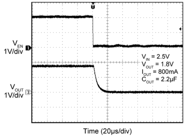
Enable Turn-Off
