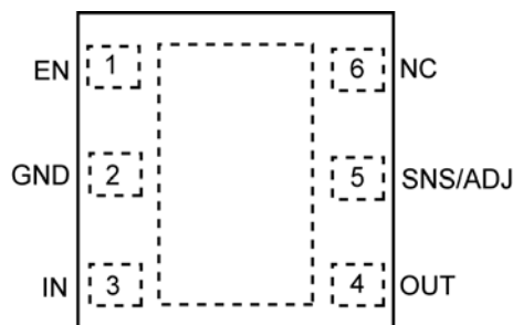
2mm x 2mm MLF ® - 6 Lead (MT) MIC371xx (Fixed/Adjustable)
