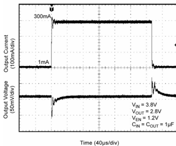
Load Transient
