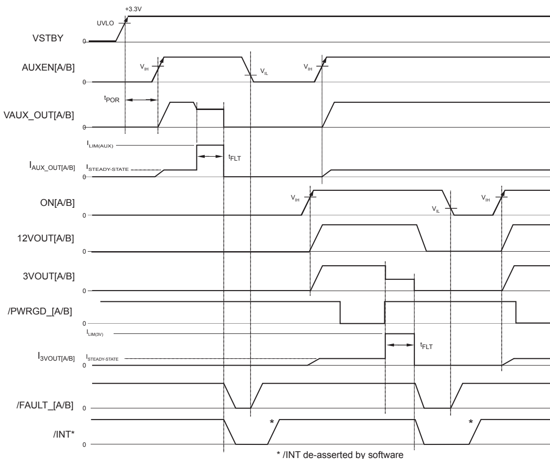
Figure 9. Hot-Plug Interface Operation
