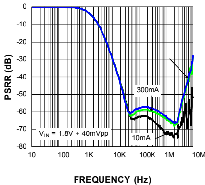
PSRR C_{OUT} = 22\mu F
