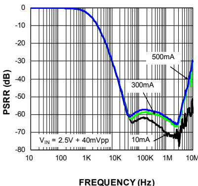
PSRR C_{OUT} = 22\mu F
