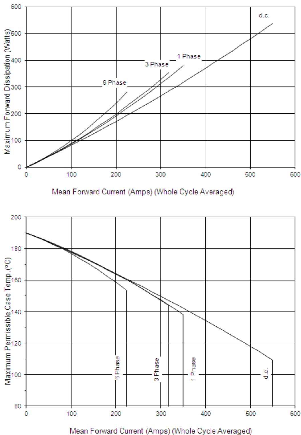
Figure 4 – Dissipation/Case temperature v Mean forward current
