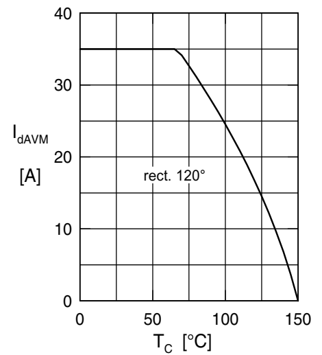
Fig. 4 Maximum forward current at case temperature T_C
