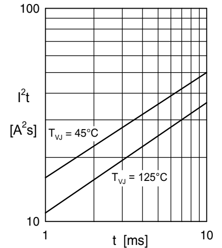
Fig. 2 I^2t versus time (1-10 ms) per diode
