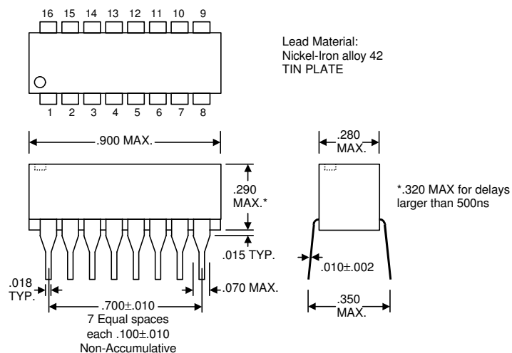
Package Dimensions
