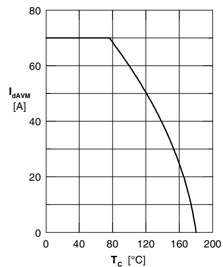
Fig. 5 Max. forward current versus case temperature, sine 180°
