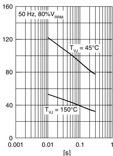
Fig. 2 Surge overload current
